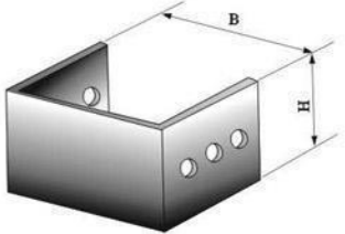
XQJ-C-01B桥架封头 XQJ-C-01B Support end piece
